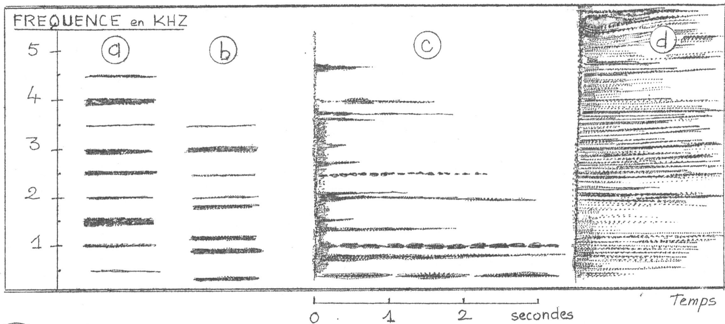
fig.3 Spectre HARMONIQUE Spectre de PARTIELS CLOCHE CYMBALE
